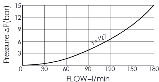
FULLY OPEN RESTRICTOR-FLOW IN BOTH DIRECTIONS
