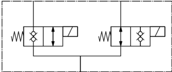
The Y=54 direct-acting, poppet-type, 3-way 2-position solenoid directional valve can replace two direct-acting, poppet-type 2-way 2-position solenoid directional valves (Y=52 and Y=51).
