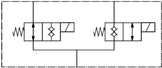
The Y=53 direct-acting, poppet-type, 3-way 2-position solenoid directional valve can replace two direct-acting, poppet-type 2-way 2-position solenoid directional valves (Y=51 and Y=52).
